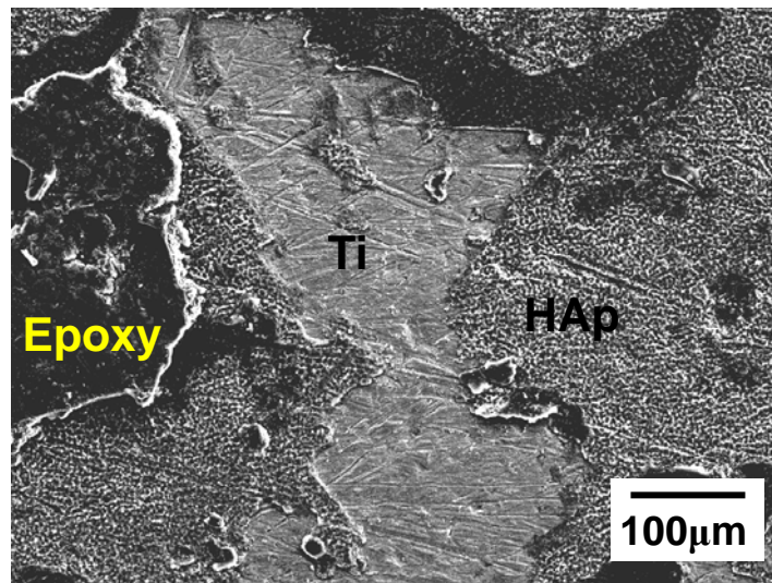
Fig. 5 Scanning electron microscopy micrograph of fracture surface of HA sample after tensile adhesion strength test; the failure occurred in epoxy, between the HAp coating and epoxy, and between Ti substrate and the HAp coating.
